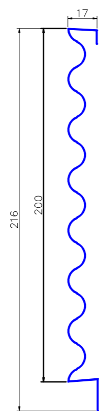
PAINEL BSM-200MW
