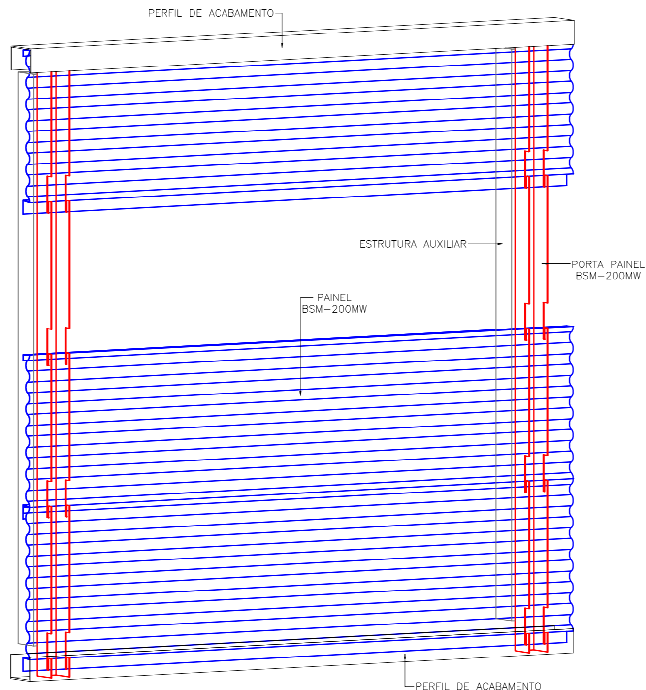
PERSPECTIVA DO PAINEL BSM-200MW
