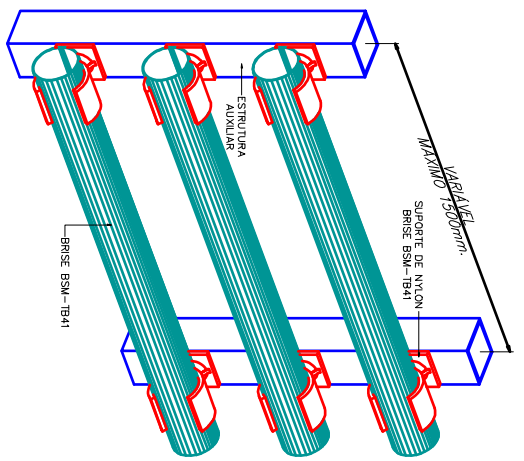
PERSPECTIVA BSM-TB41
